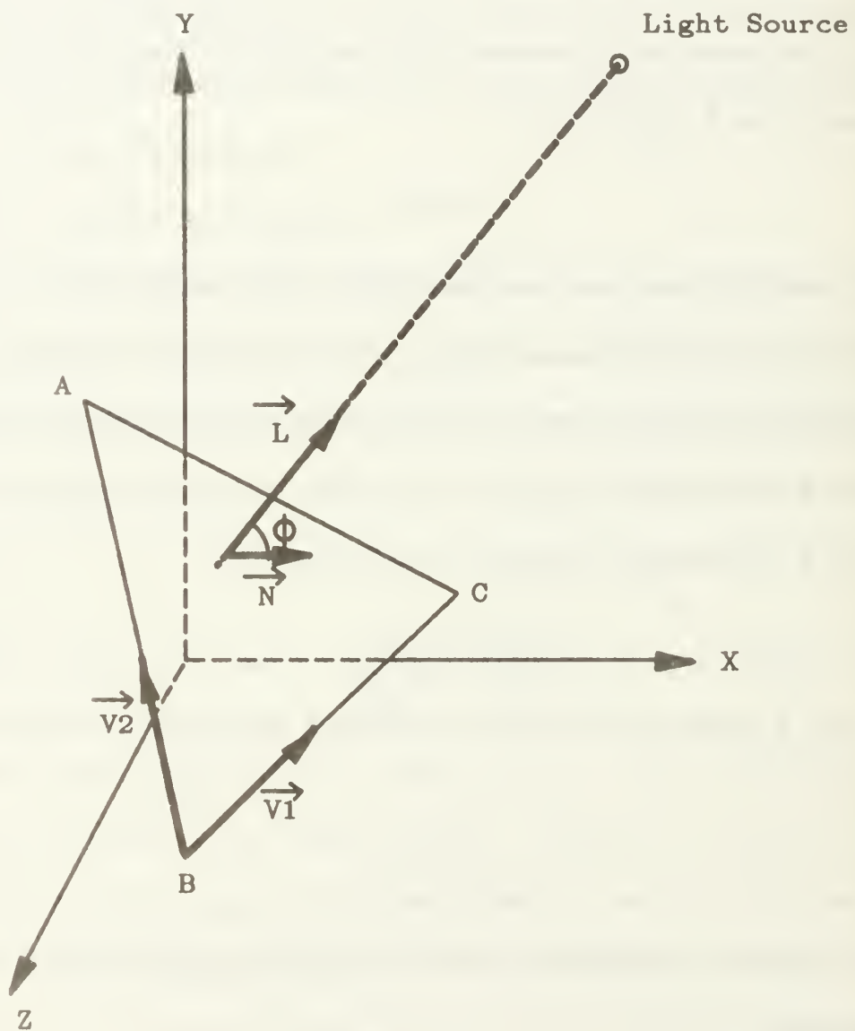
Figure 5.2 Lambert's Cosine Law
